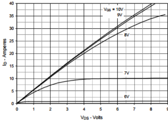
Fig. 3. Output Characteristics @ T_J = 125^\circ\text{C}
