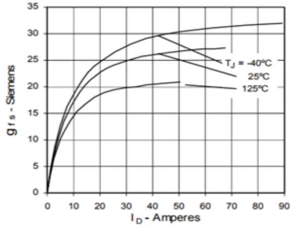
Fig. 8. Transconductance
