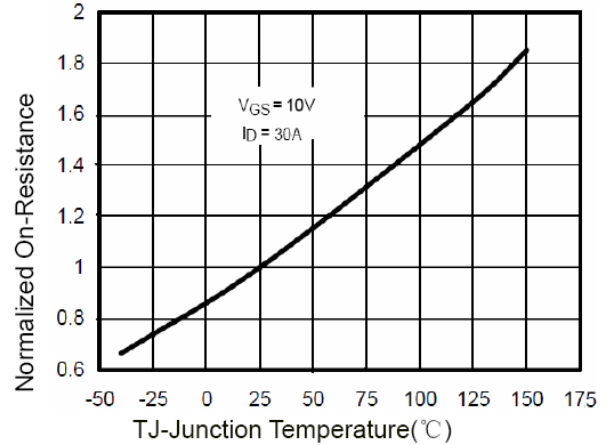
Figure 4 Rdson-Junction Temperature
