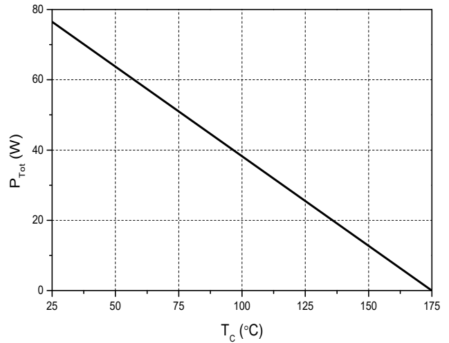
Figure 6. Power Derating
