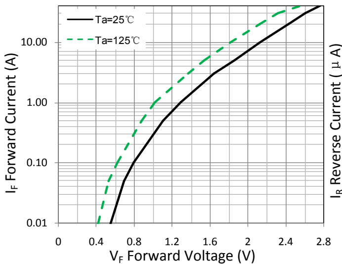
Figure 1. Forward Characteristic(typ.)
