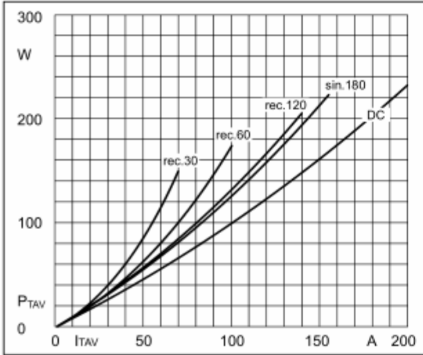
Fig1. Power dissipation
