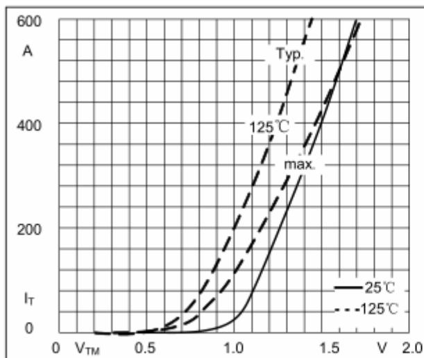
Fig5. Forward Characteristics
