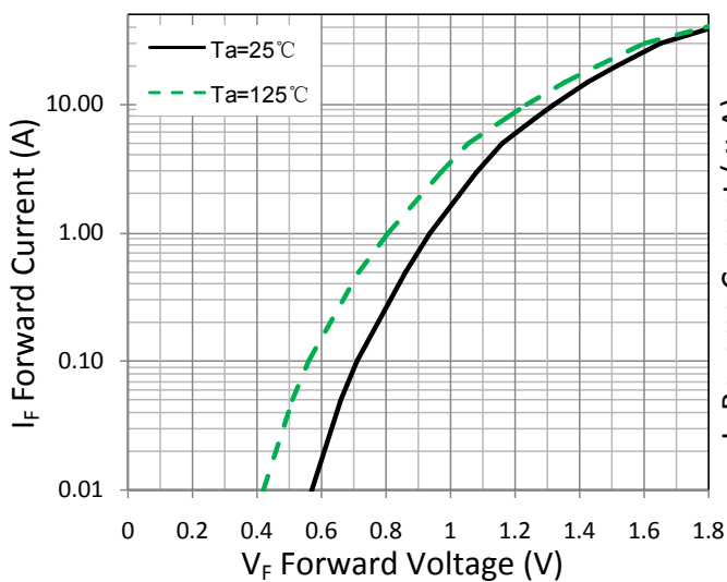
Figure 1. Forward Characteristic(typ.)
