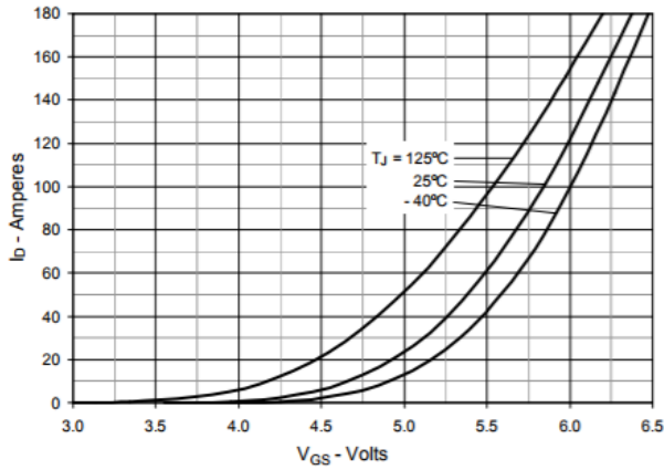
Fig. 7. Input Admittance
