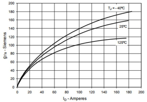
Fig. 8. Transconductance
