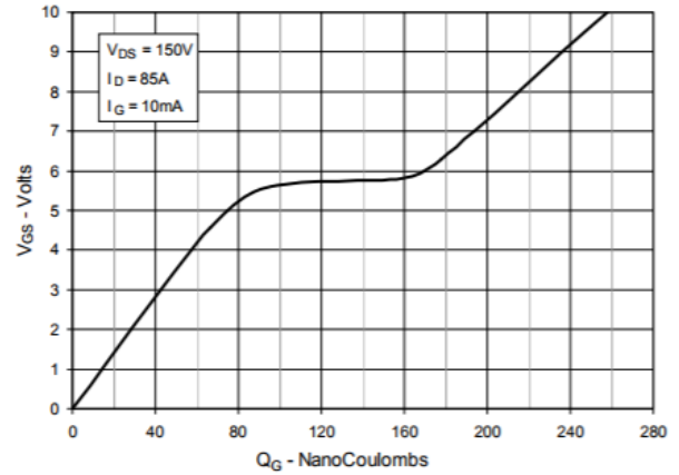
Fig. 10. Gate Charge
