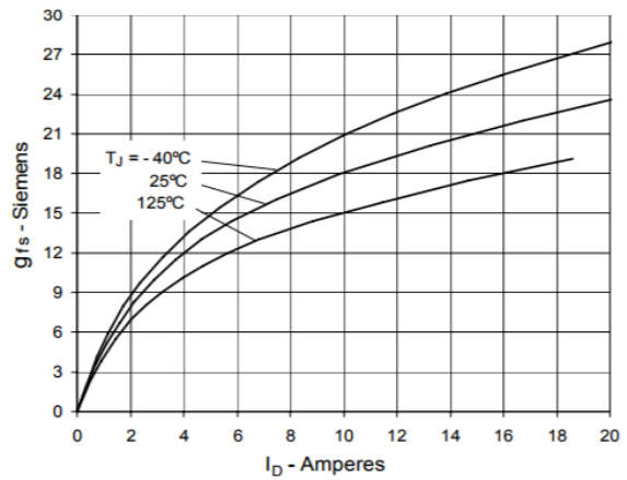
Fig. 8. Transconductance
