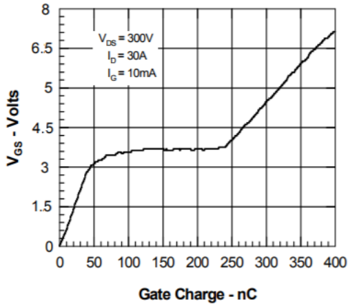
Figure 7. Gate Charge
