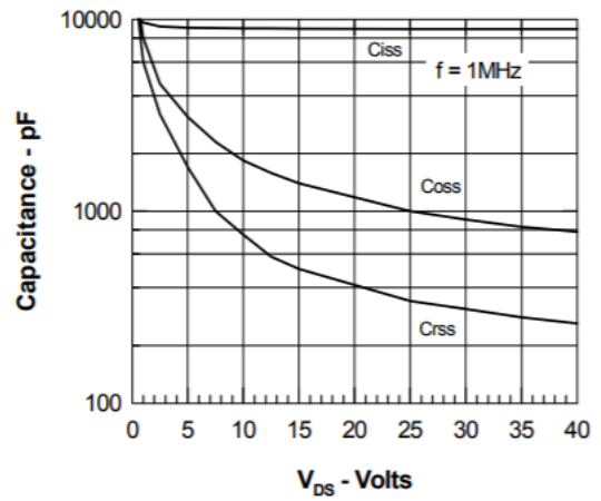
Figure 8. Capacitance Curves
