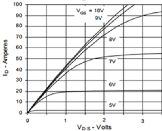
Fig. 3. Output Characteristics @ 150°C
