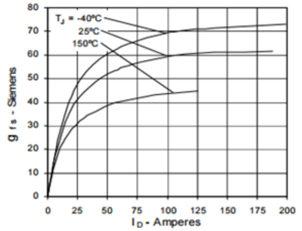
Fig. 8. Transconductance
