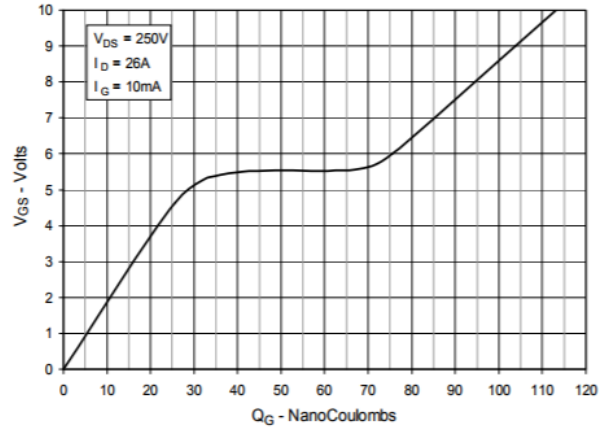
Fig. 10. Gate Charge
