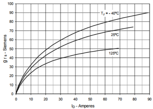
Fig. 8. Transconductance
