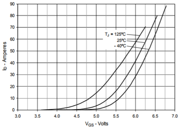
Fig. 7. Input Admittance
