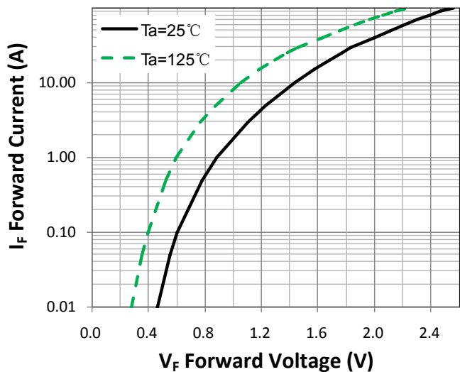
Figure 1. Forward Characteristic(typ.)
