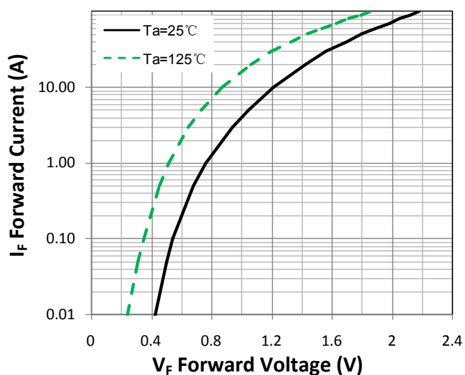
Figure 1. Forward Characteristic(typ.)
