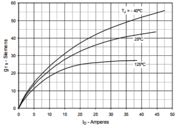
Fig. 8. Transconductance
